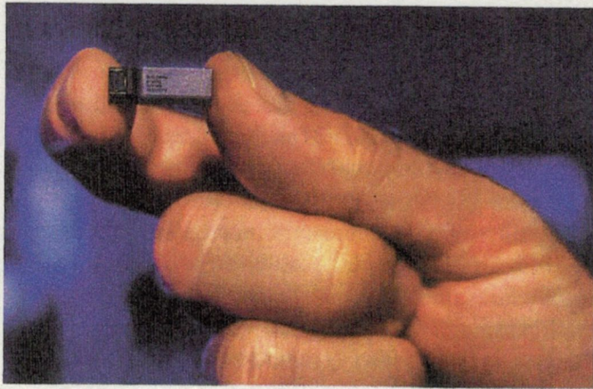
FIGURE 4. Qualcomm's millimetre wave antenna array module for a 5G smartphone. It has four antennas that can accurately point towards the nearest 5G base station. Phones will have four of these modules, i.e. sixteen antennas. 4
